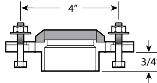
HUB or FPT with 4" centre
