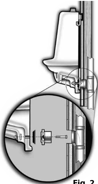
Fig. 2 Side exploded detail
