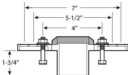
Spigot with adjustable 4" - 7" centres
