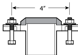
Spigot with 4" centre
